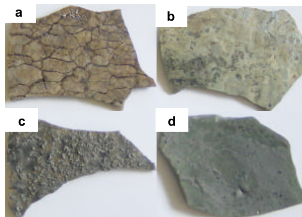
Fig.1 The appearance of mould flux films A and B. a, b: the surface against mould of samples A and B; c, d: the surface against shell of samples A and B.
