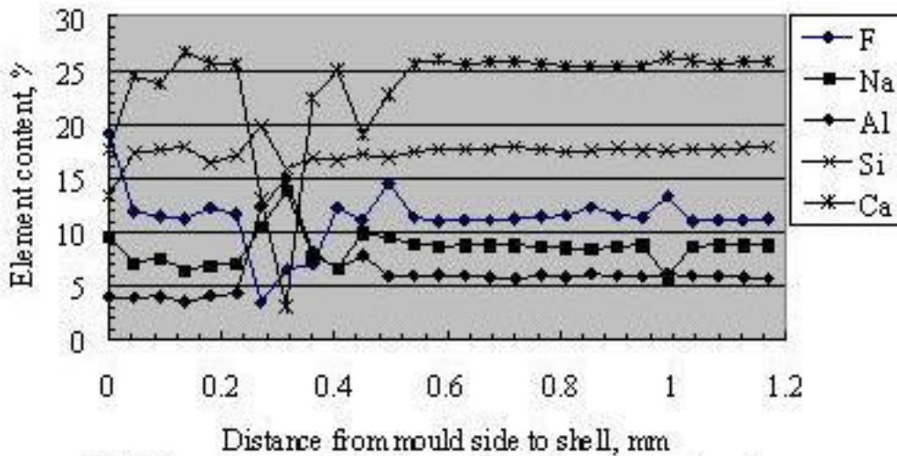
Fig 7 – Element Concentration change along the cross section of mould flux film B
